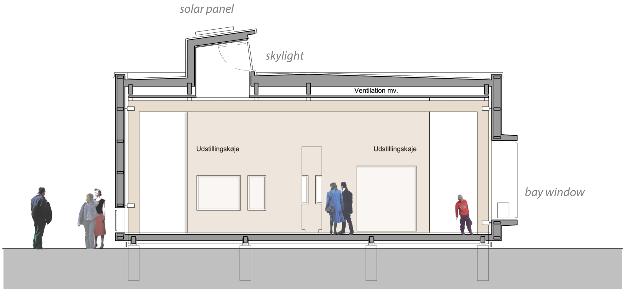
Exhibition space cross-section
