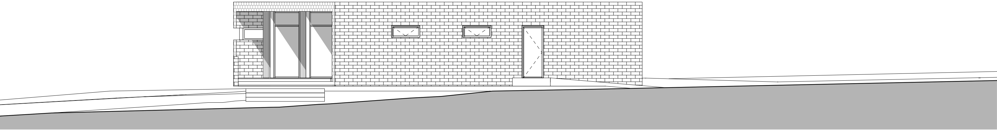
ELEVATION WEST
