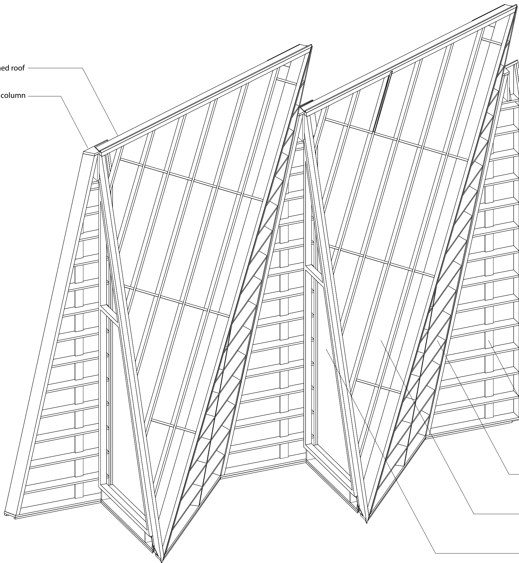
3D PRE-FAB CLADDING MODULES - EXTERIOR VIEW
