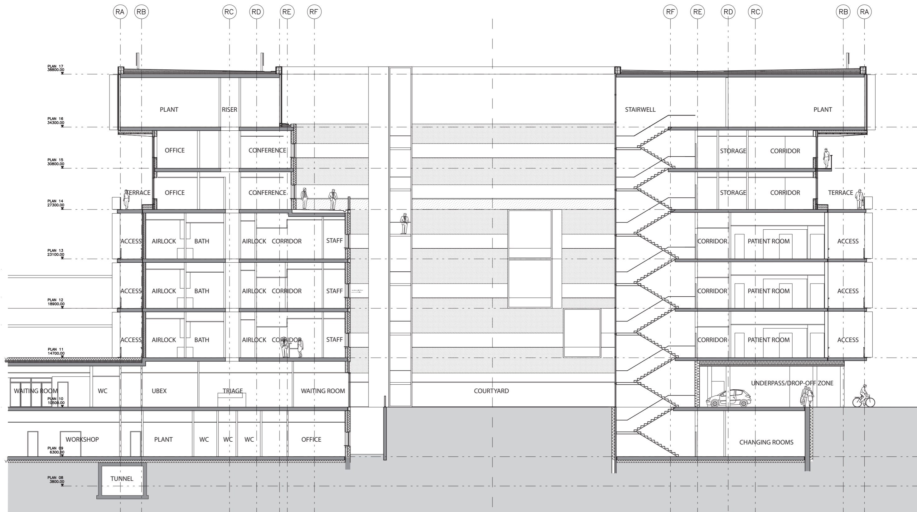
CROSS SECTION 1:200 @ A3
