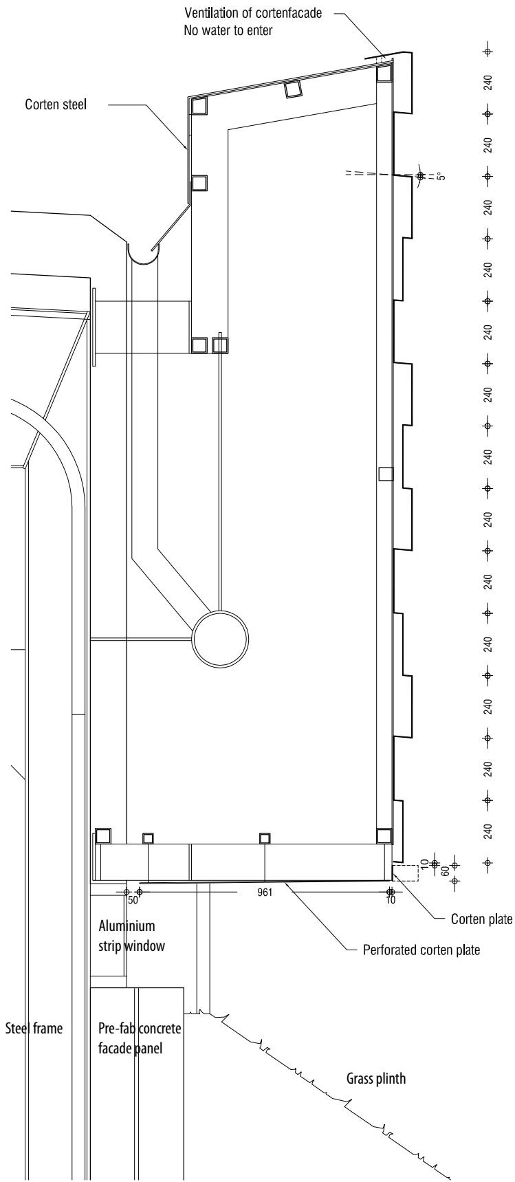
Section 1, No gutter and bottom plate
