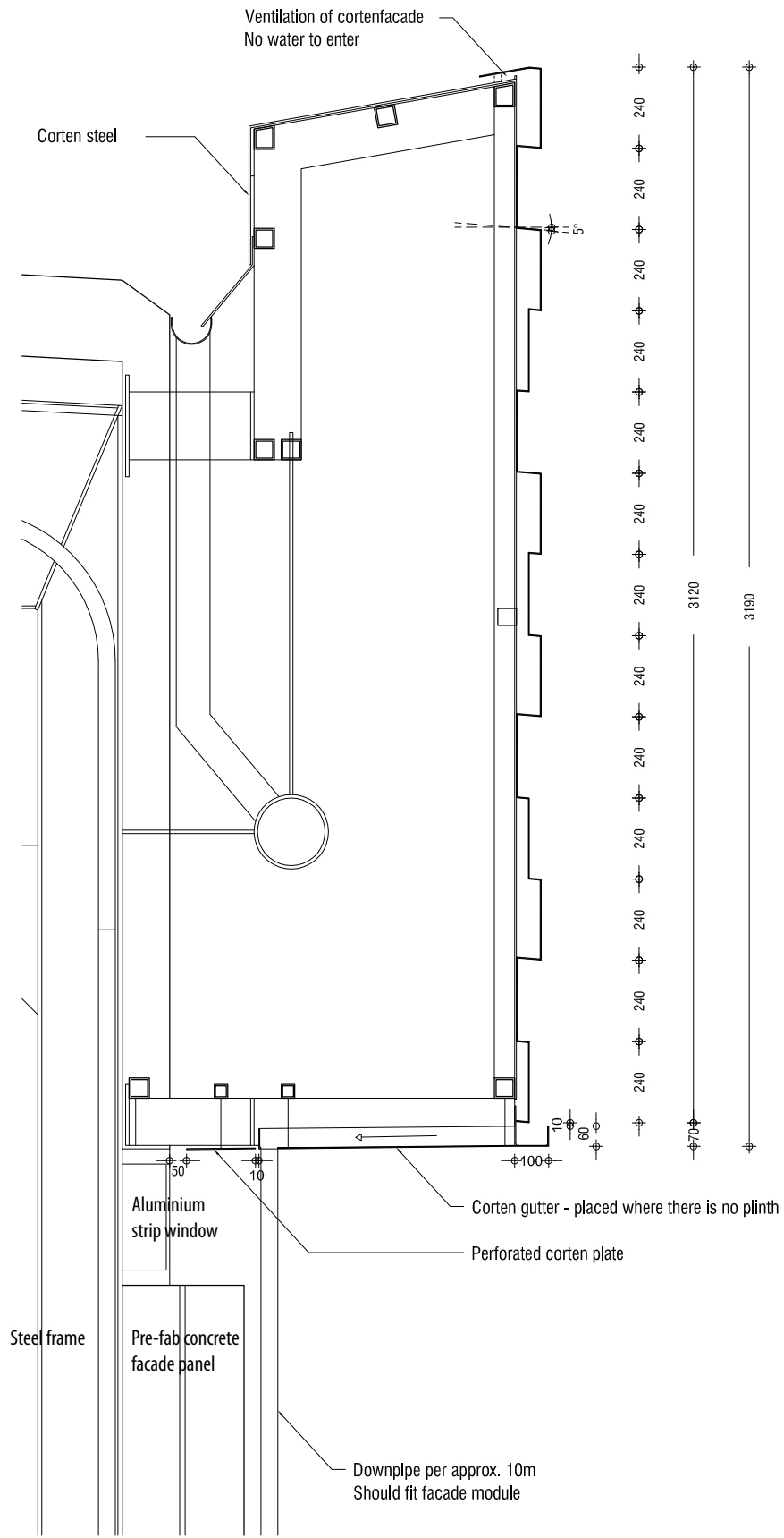
Section 2, Main gutter and gutter to downpipe
