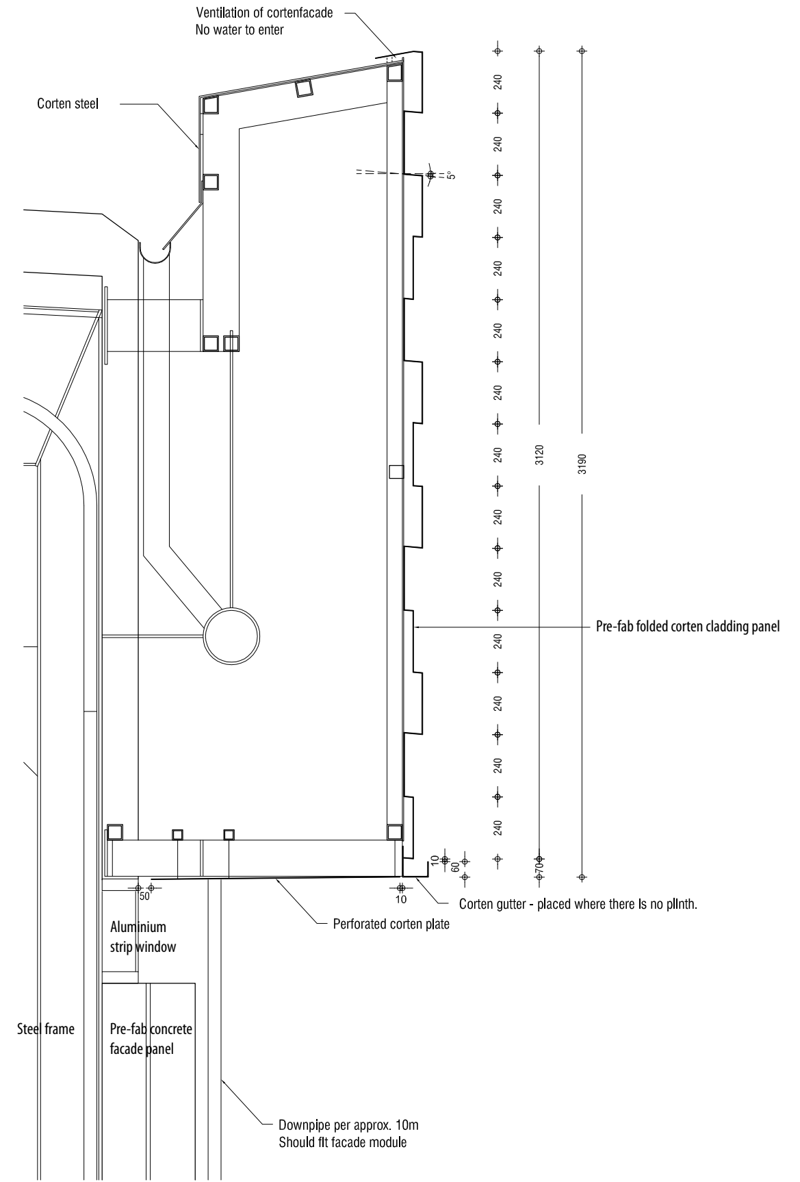
Section 3, Main gutter and bottom plate
