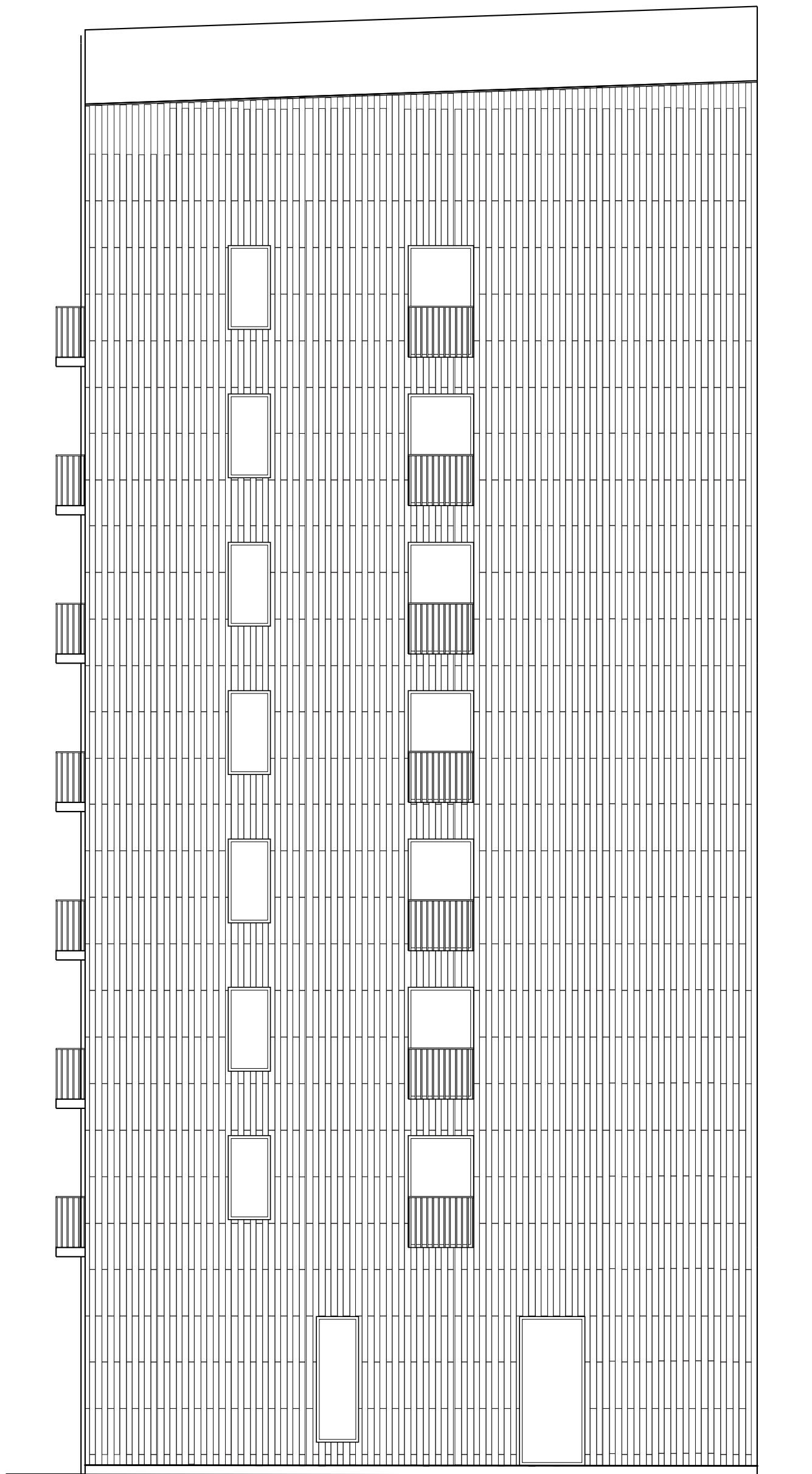
Facade North, 9-storey timber building - Scale 1:100
