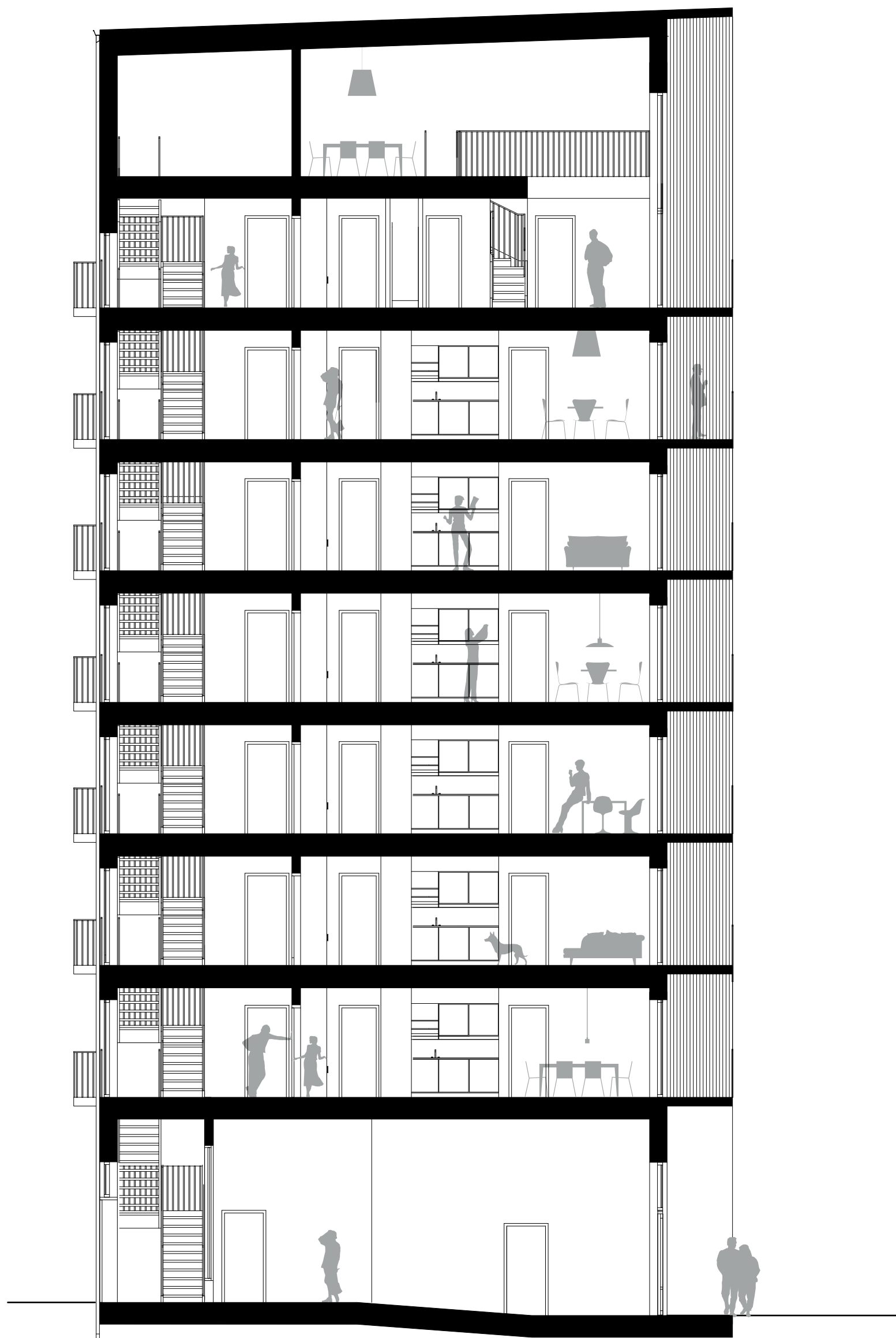
Section B-B, 9-storey timber building - Scale 1:100
