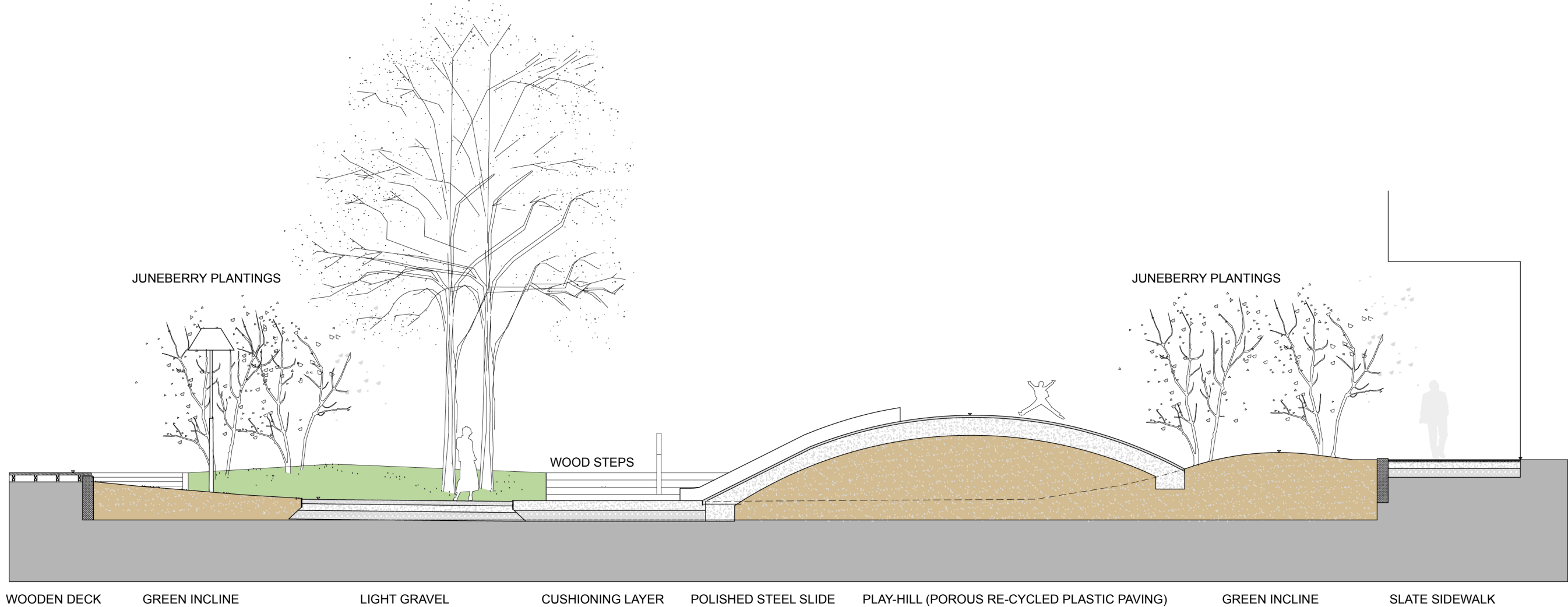
CROSS-SECTION PLAYGROUND JOMFRU ANE PARK
