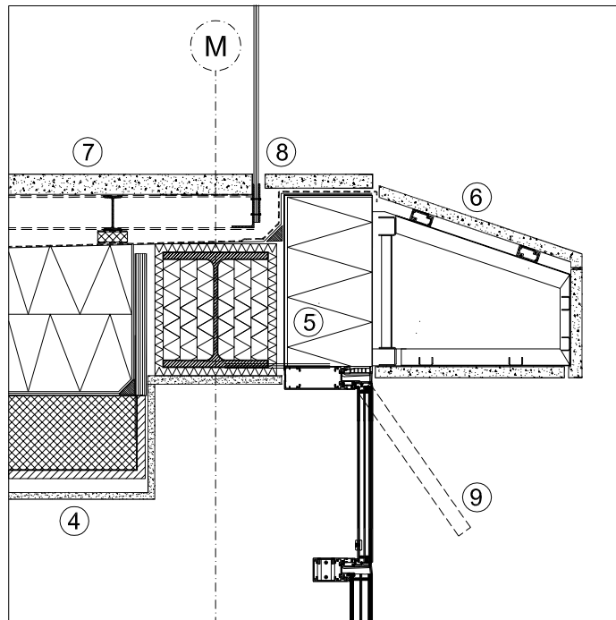
VERTICAL SECTION - ROOF TERRACE
