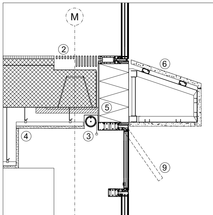
VERTICAL SECTION - FLOORSLABS
