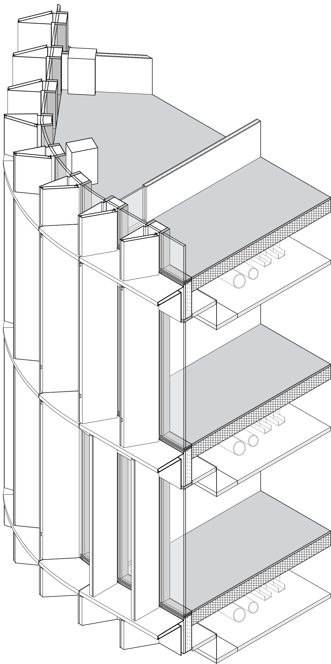
Isometric detail of facade shutters 1:50
