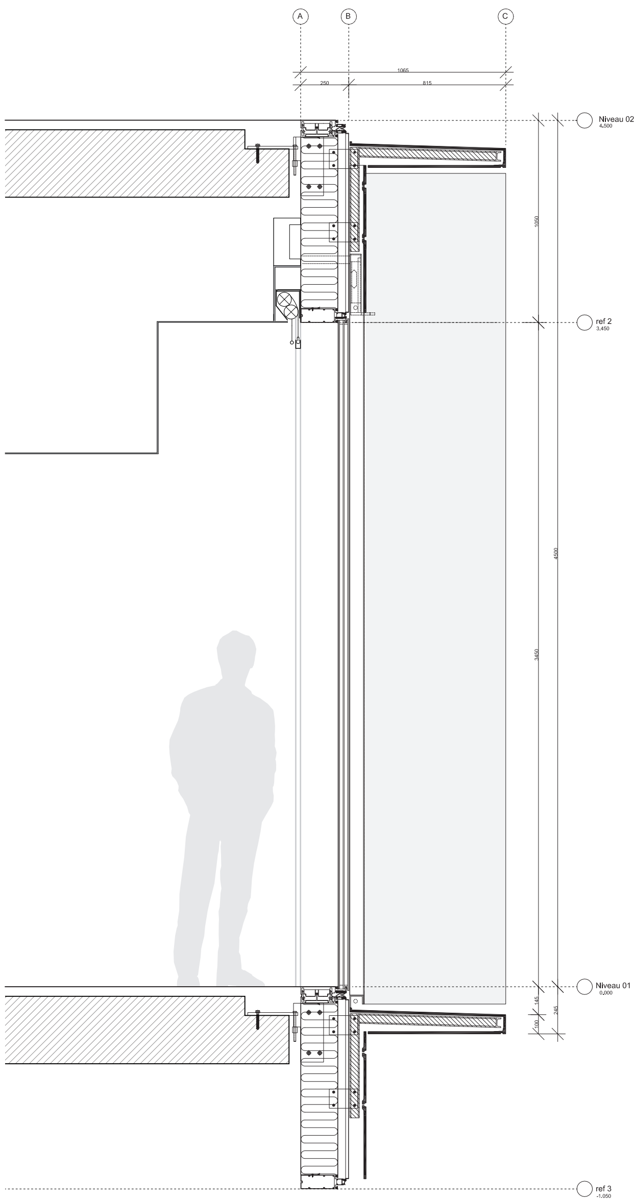
Section detail of facade shutters 1:20
